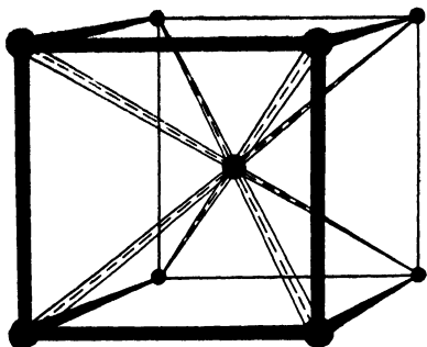
FIG. 3.—A unit-cube from a body-centered cubic lattice.
